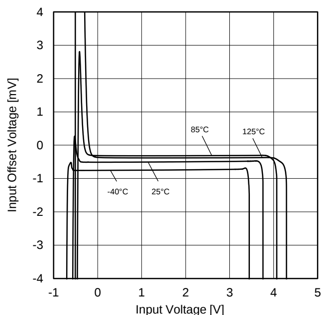
Figure 15. Input Offset Voltage vs Input Voltage ( V_{CC}=5V )
