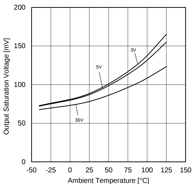
Figure 4. Output Saturation Voltage vs Ambient Temperature ( I_{\text{SINK}}=4\text{mA} )
