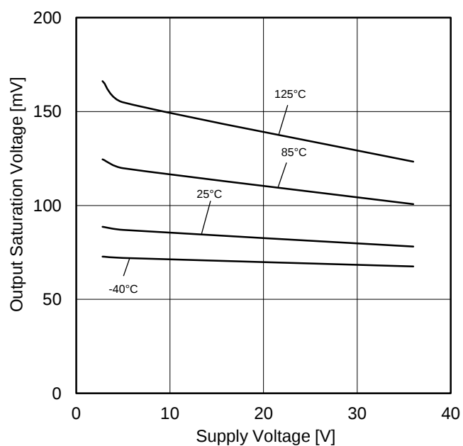
Figure 3. Output Saturation Voltage vs Supply Voltage ( I_{\text{SINK}}=4\text{mA} )
