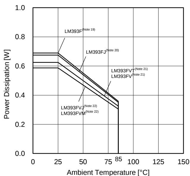
(c) LM393xxx
